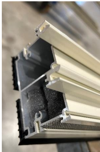
Machined profile and EPDM joint
